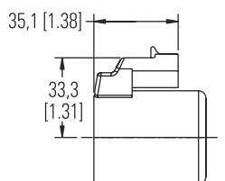
D0 Metri-Pack 150 Male, integrated connector
