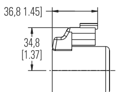
N0 Deutsch male DTO4-2P integrated connector
