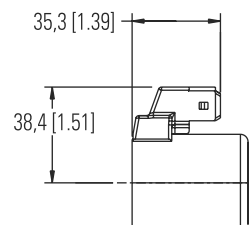
Y0 AMP Junior timer integrated connector
