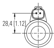
N0 Deutsch male DTO4-2P integrated connector
