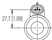
D0 Metri-Pack 150 Male, integrated connector
