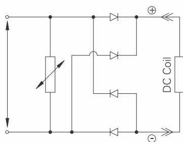
AC Voltage Connector Circuit Diagram
