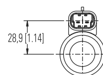
J0 Metri-Pack 280 Male, integrated connector
