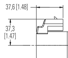
J0 Metri-Pack 280 Male, integrated connector
