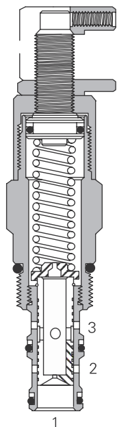
Sectional view
