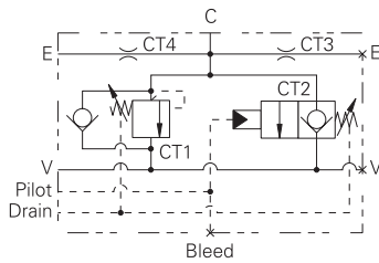
Typical circuit
