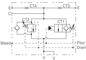
Typical circuit
