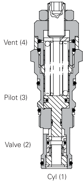
Sectional view
