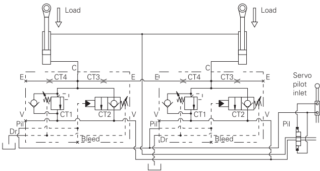
Typical circuit
