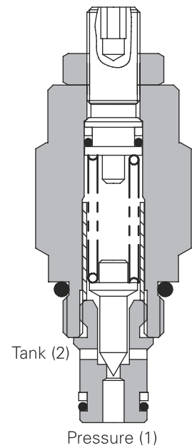
Sectional view
