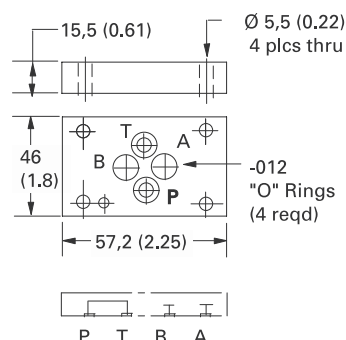
Linking plate 02-185278
