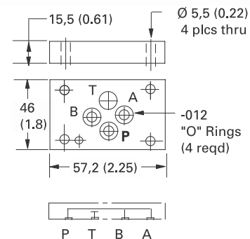
Linking plate 02-185281
