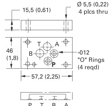
Linking plate 02-185275
