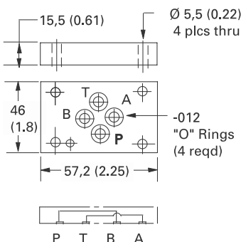
Linking plate 02-185277
