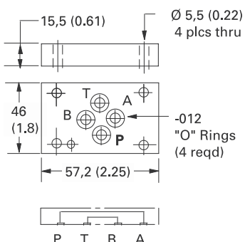
Linking plate 02-185276
