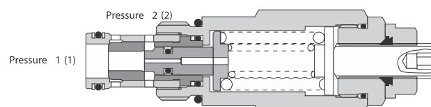
Figure 8. 1CLLR50 Dual relief
